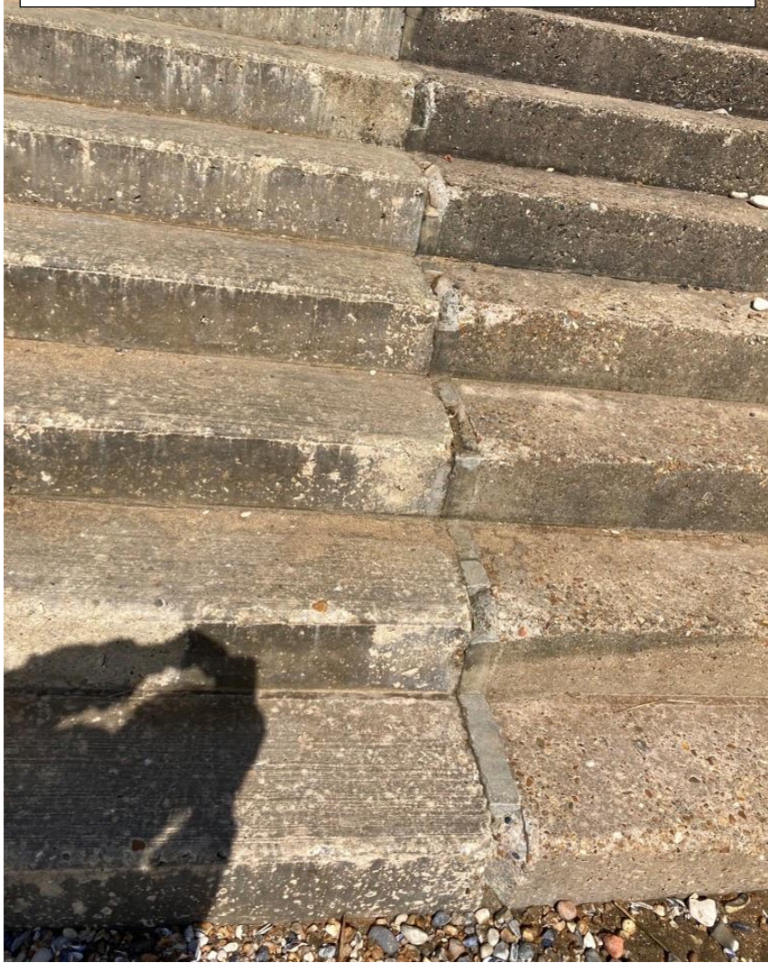
Wave-return wall before mortar joint replacement
